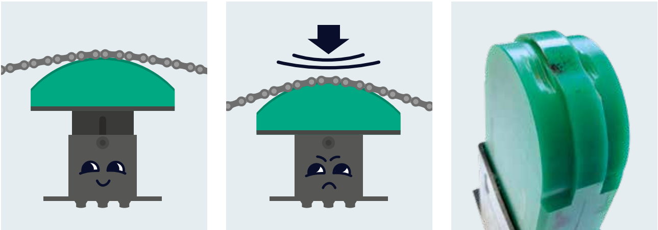
Possible wear patterns caused by overloading the Spann-Box®
